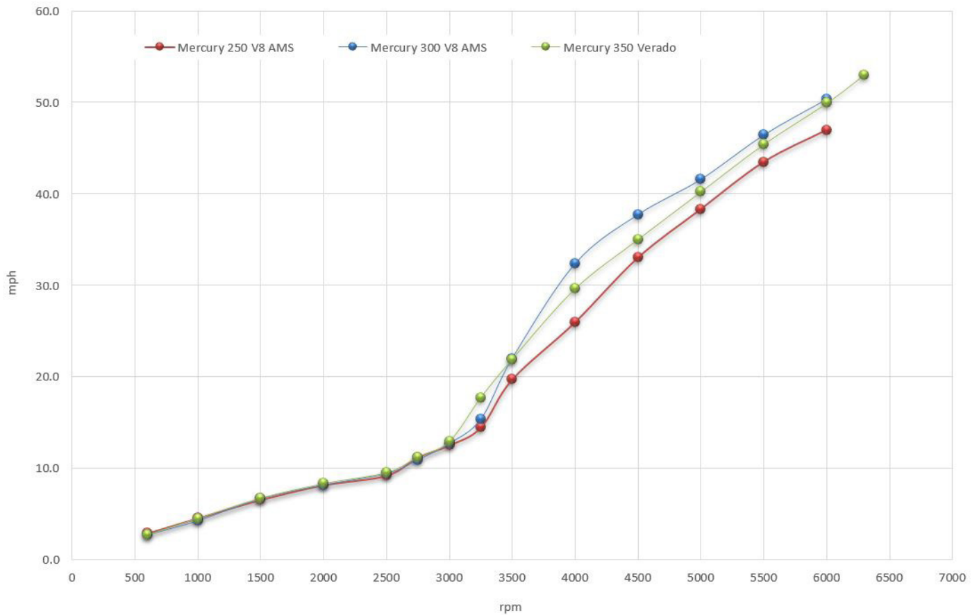
230 Vantage Engine Comparison Graph
