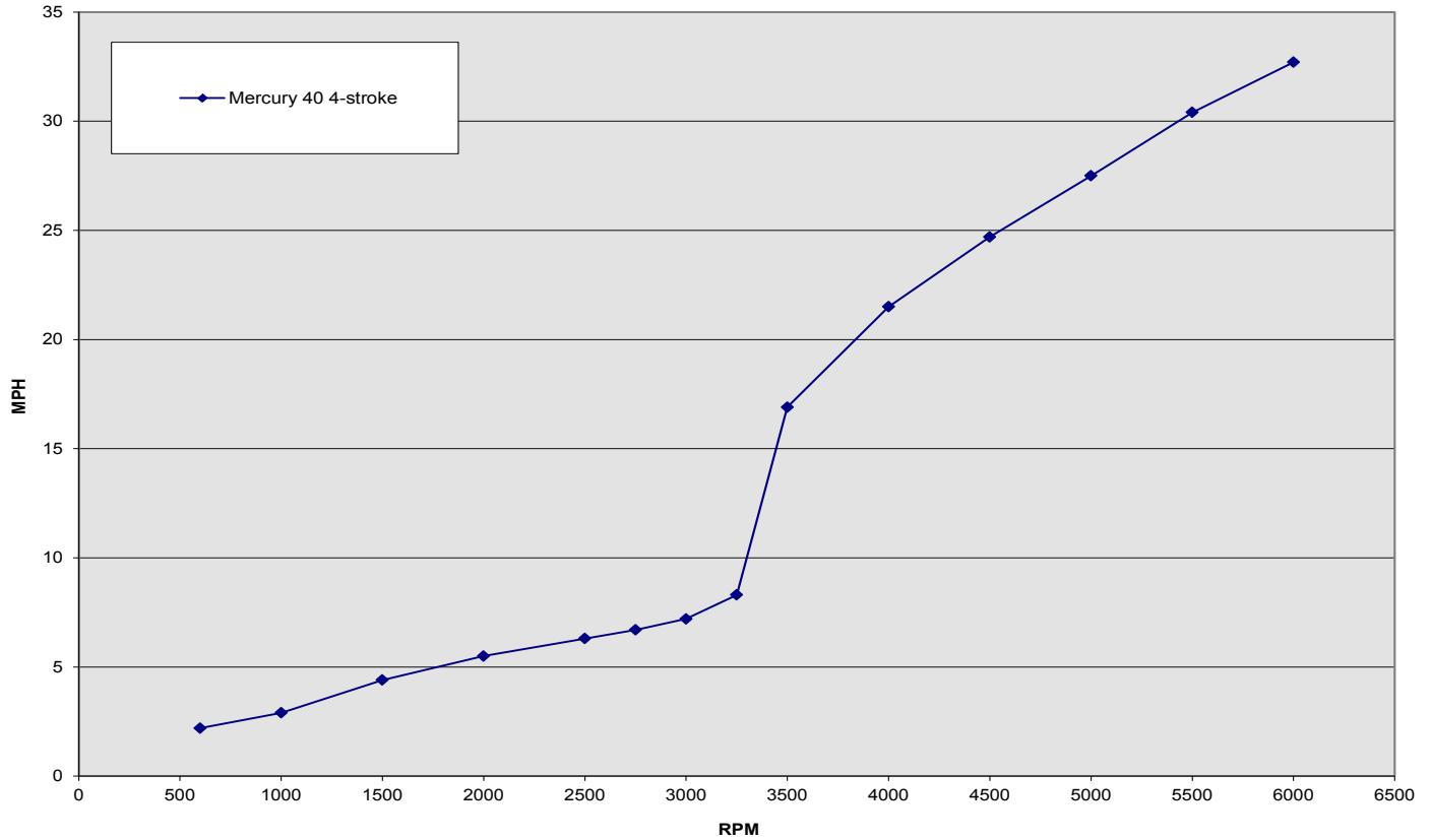
130 Super Sport Engine Comparison Graph
